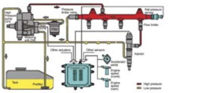
DOOSAN DLo8 "Common-Rail" Motor
